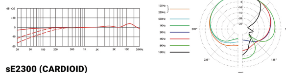
sE2300 (CARDIOID)
